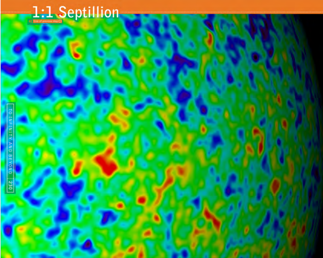
Cosmic Microwave Background
