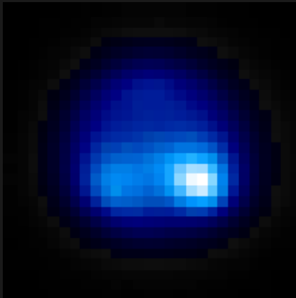
Neptune
