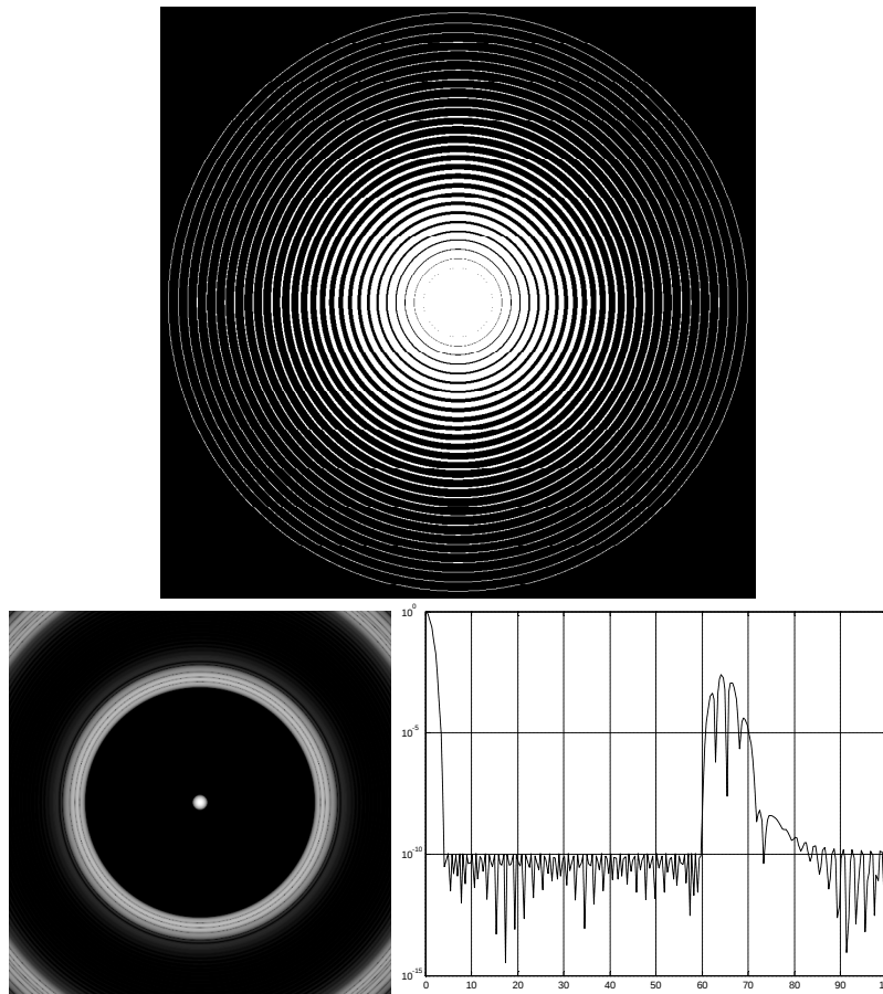
Figure 7.6. At the top is shown the concentric ring apodization. The second row shows the psf as a 2-D image and in cross-section. Note that it achieves the required 10^{-10} level of darkness at a distance of only 4 from the center of the Airy disk.
