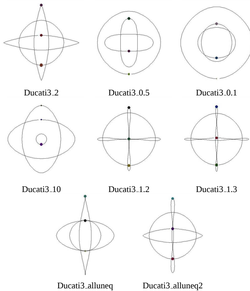
Figure 7.15. Periodic Orbits—Ducati's with unequal masses.
