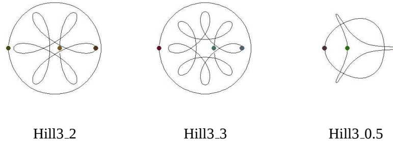
Figure 7.14. Periodic Orbits—Hill-type with equal masses.
