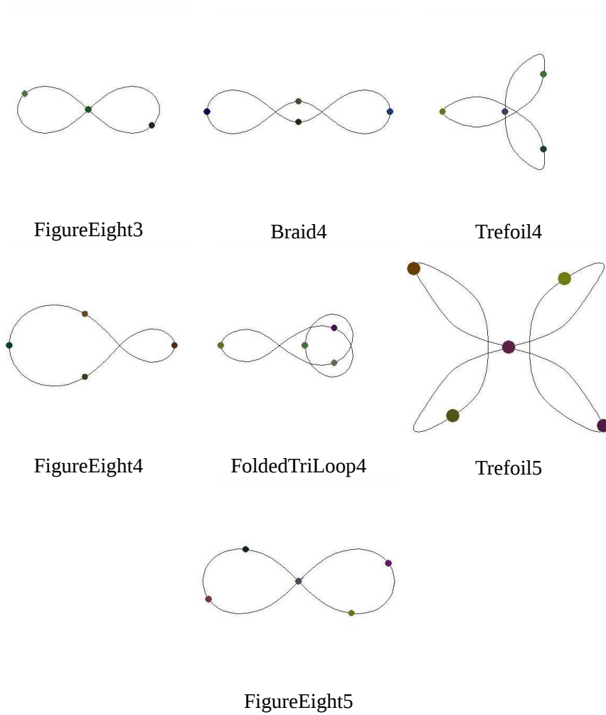
Figure 7.12. Periodic Orbits—Choreographies.
