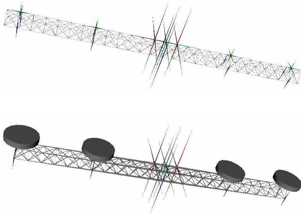
Figure 7.9. Top. The design space. Bottom. The optimal design.
