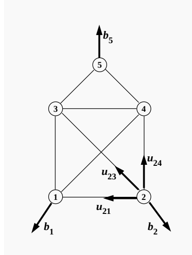
Figure 7.7. A design space showing 5 nodes and 8 arcs. Also shown are three externally applied forces and the tensile forces they induce in node 2.
