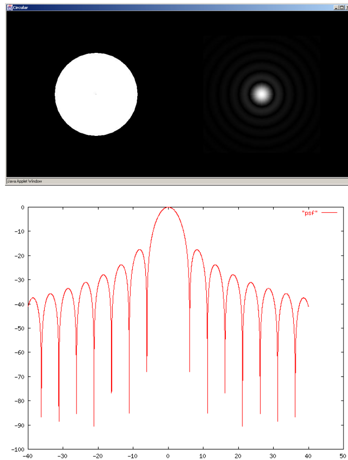
Figure 7.4. The top left shows a circular opening at the front of a telescope. The top right shows the corresponding Airy disk and a few diffraction rings. The plot on the bottom shows the cross-sectional intensity on a log scale. The desired level of 10^{-10} corresponds to an intensity level of -100 on this log plot. It is way off to the side. It occurs out somewhere around the 100th diffraction ring.
