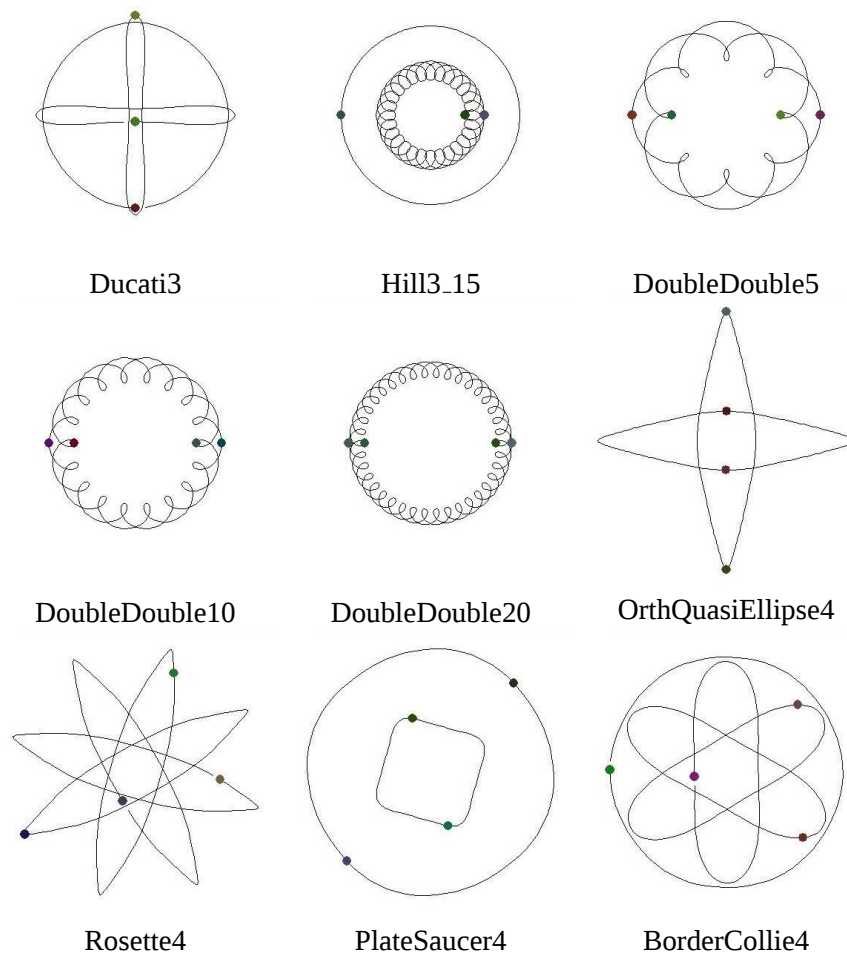
Figure 7.13. Periodic Orbits–Non-Choreographies.
