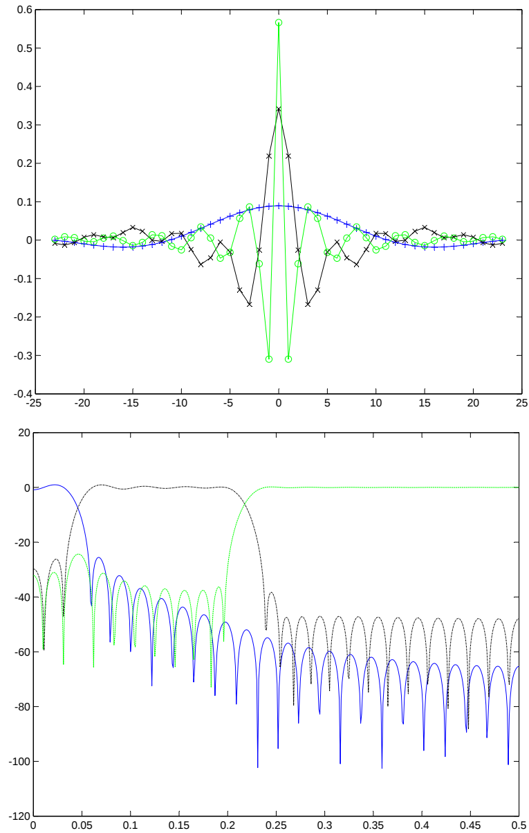
Figure 7.3. Top. The optimal filter coefficients. Bottom. The corresponding spectral response curves. In the top graph, the \circ 's correspond to the tweeter filter, the \times 's correspond to the midrange filter, and the + 's correspond to the woofer filter. The spectral response curve is a plot of ten times log base ten of power as a function of frequency.
